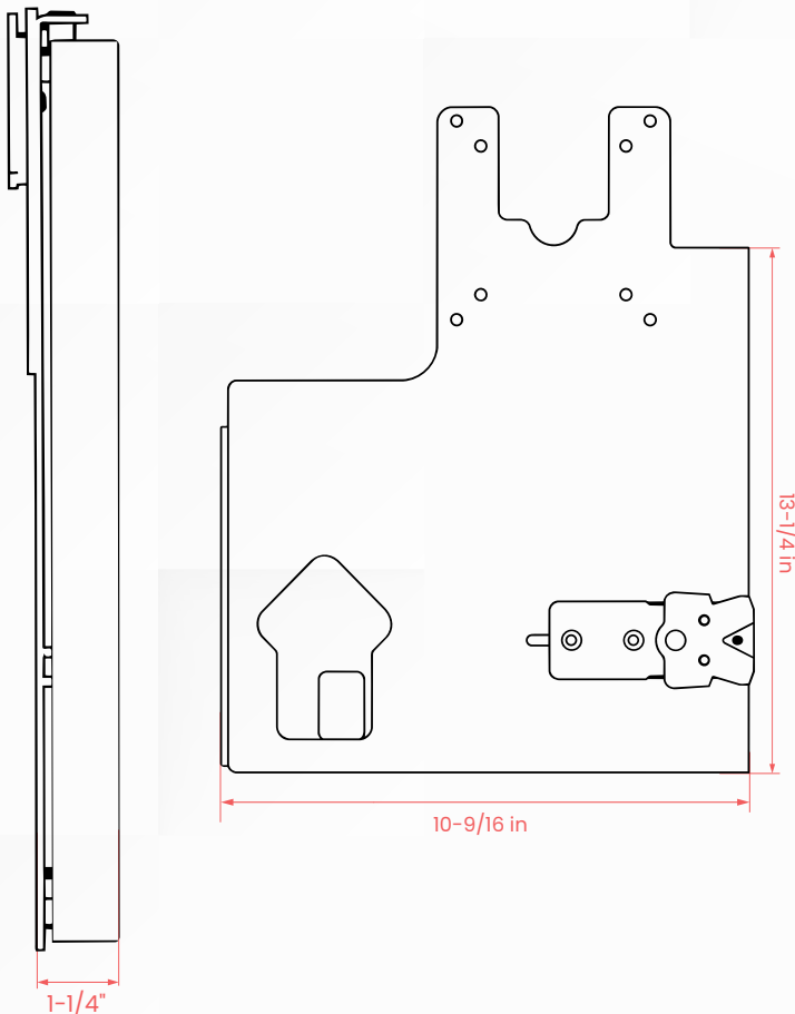
PAYMENT TERMINAL HEIGHT ADJUSTMENT
