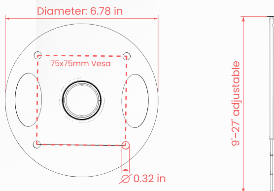
VESA Canopy Mounting Plate
