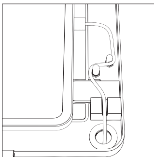
**Tablet and cable only shown for illustration purposes, not included. 2A. Internal cable routing.
